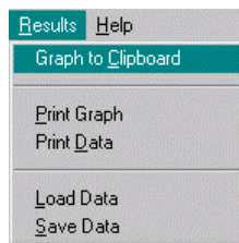
Fig. 5 Results Menu
